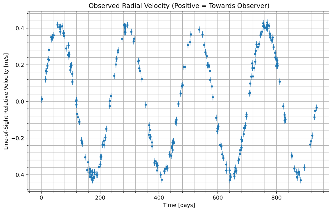
Figure 1: We have isolated the radial velocity of the host star due to the candidate planet. Data begins at UTC 2079-11-18/07:24. Positive values indicate the velocity at which the star is moving towards us; negative indicate the velocity at which it is moving away.
