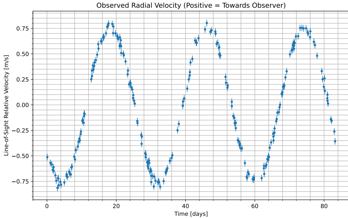
Figure 1: We have isolated the radial velocity of the host star due to the candidate planet. Data begins at UTC 2084-09-29/00:03. Positive values indicate the velocity at which the star is moving towards us; negative indicate the velocity at which it is moving away.
