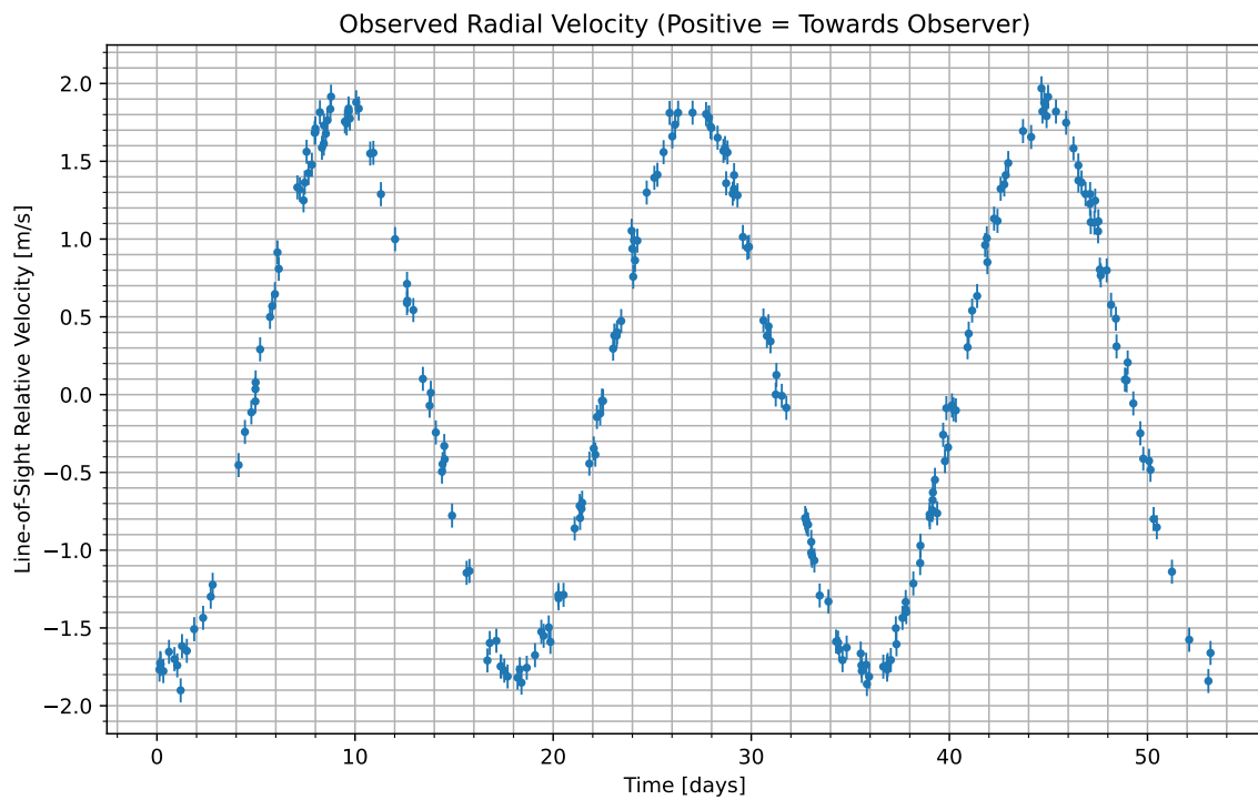
Figure 1: We have isolated the radial velocity of the host star due to the candidate planet. Data begins at UTC 2082-05-06/16:01. Positive values indicate the velocity at which the star is moving towards us; negative indicate the velocity at which it is moving away.
