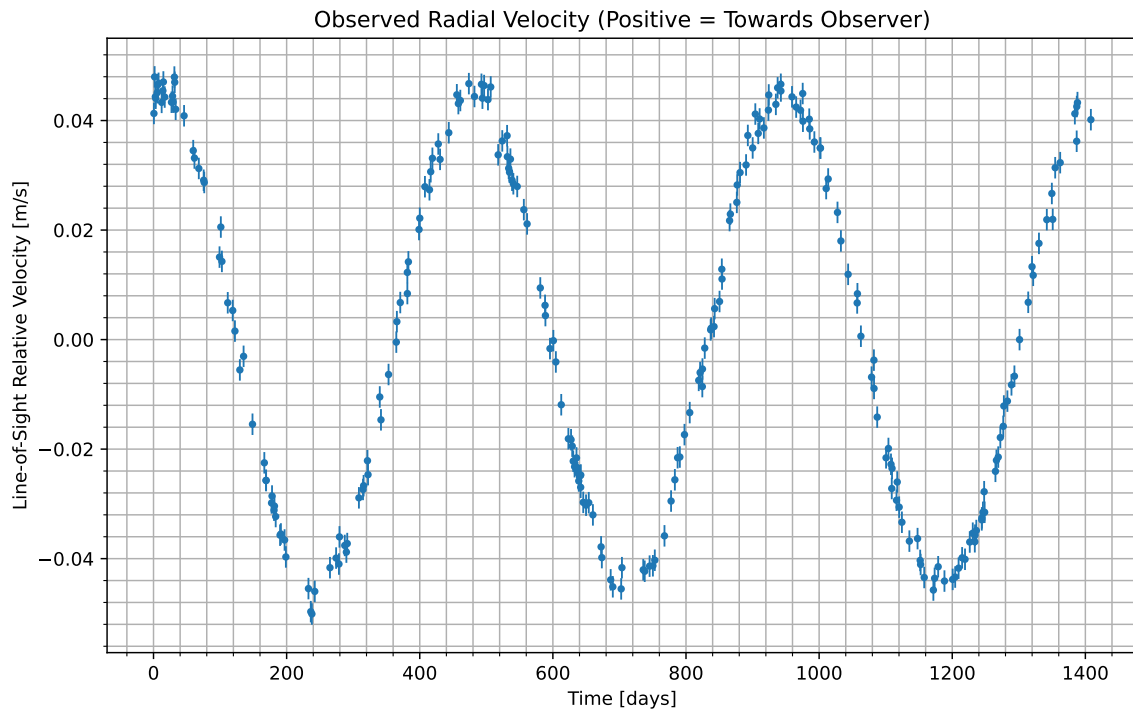
Figure 1: We have isolated the radial velocity of the host star due to the candidate planet. Data begins at UTC 2096-10-21/01:10. Positive values indicate the velocity at which the star is moving towards us; negative indicate the velocity at which it is moving away.
