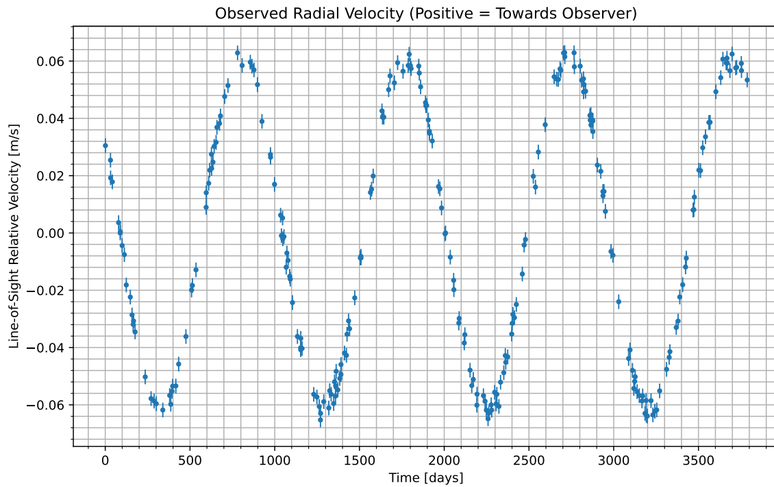
Figure 1: We have isolated the radial velocity of the host star due to the candidate planet. Data begins at UTC 2071-05-13/23:04. Positive values indicate the velocity at which the star is moving towards us; negative indicate the velocity at which it is moving away.
