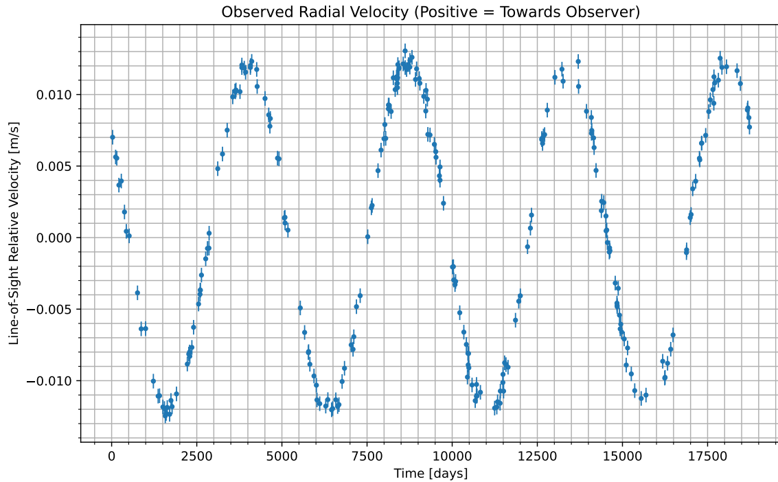
Figure 1: We have isolated the radial velocity of the host star due to the candidate planet. Data begins at UTC 2023-08-07/01:21. Positive values indicate the velocity at which the star is moving towards us; negative indicate the velocity at which it is moving away.
