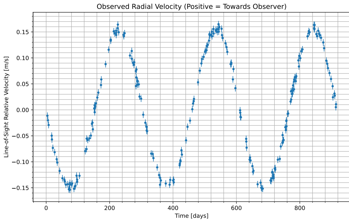
Figure 1: We have isolated the radial velocity of the host star due to the candidate planet. Data begins at UTC 2077-04-06/03:50. Positive values indicate the velocity at which the star is moving towards us; negative indicate the velocity at which it is moving away.
