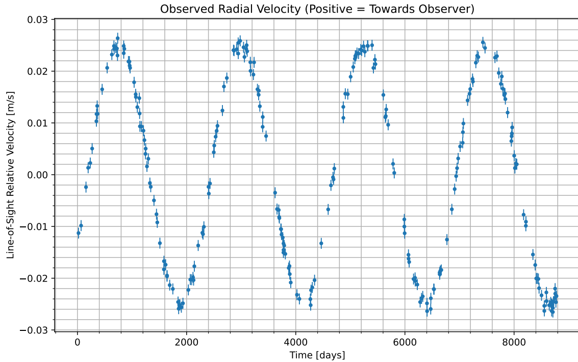
Figure 1: We have isolated the radial velocity of the host star due to the candidate planet. Data begins at UTC 2066-02-18/05:31. Positive values indicate the velocity at which the star is moving towards us; negative indicate the velocity at which it is moving away.
