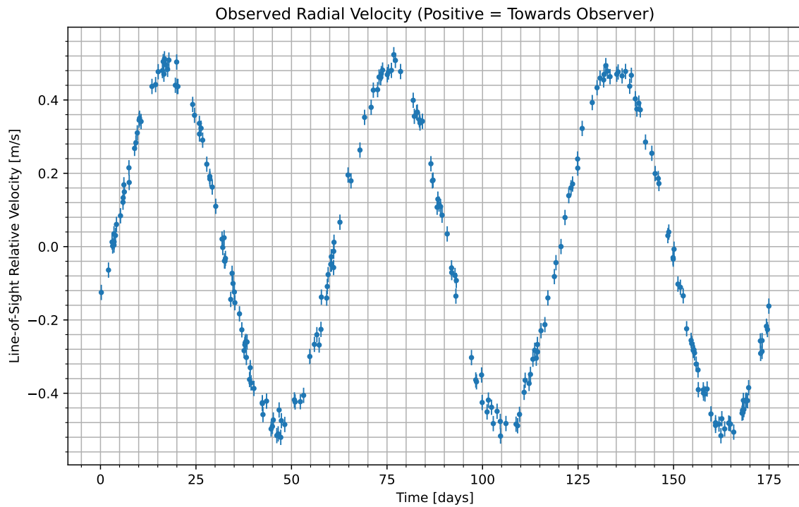
Figure 1: We have isolated the radial velocity of the host star due to the candidate planet. Data begins at UTC 2096-10-06/06:50. Positive values indicate the velocity at which the star is moving towards us; negative indicate the velocity at which it is moving away.
