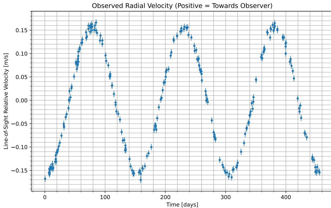
Figure 1: We have isolated the radial velocity of the host star due to the candidate planet. Data begins at UTC 2069-10-15/15:26. Positive values indicate the velocity at which the star is moving towards us; negative indicate the velocity at which it is moving away.
