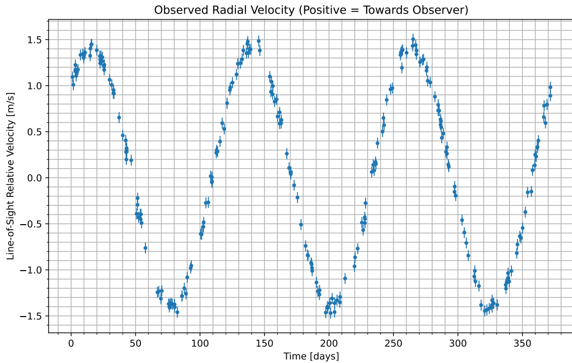
Figure 1: We have isolated the radial velocity of the host star due to the candidate planet. Data begins at UTC 2077-05-17/18:09. Positive values indicate the velocity at which the star is moving towards us; negative indicate the velocity at which it is moving away.
