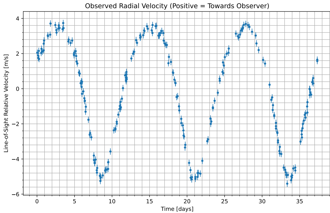
Figure 1: We have isolated the radial velocity of the host star due to the candidate planet. Data begins at UTC 2091-06-26/22:21. Positive values indicate the velocity at which the star is moving towards us; negative indicate the velocity at which it is moving away.
