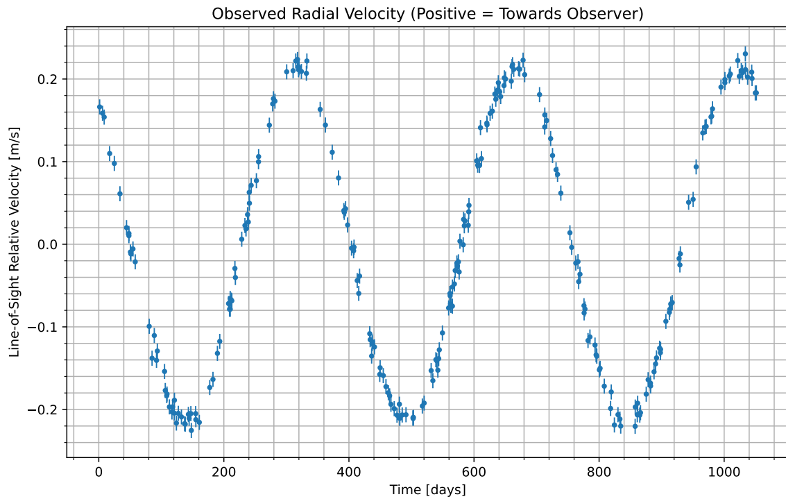
Figure 1: We have isolated the radial velocity of the host star due to the candidate planet. Data begins at UTC 2085-01-18/21:58. Positive values indicate the velocity at which the star is moving towards us; negative indicate the velocity at which it is moving away.
