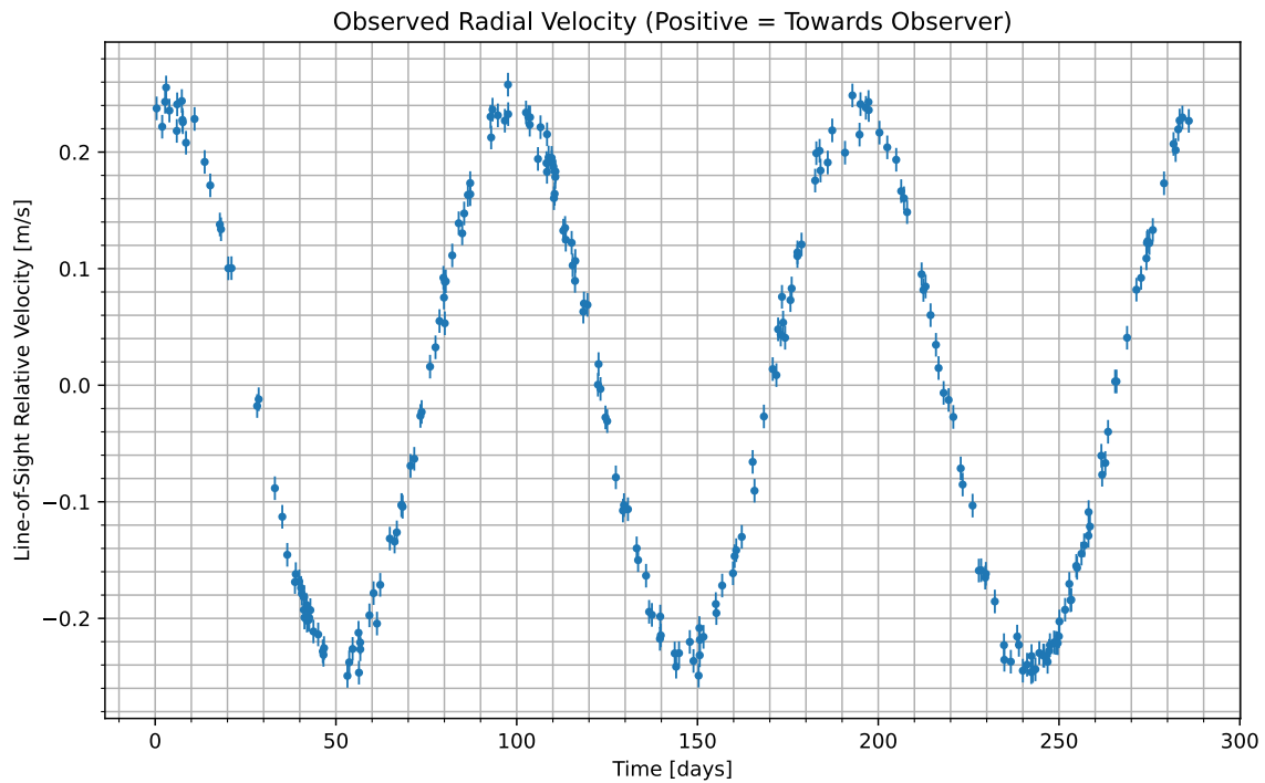
Figure 1: We have isolated the radial velocity of the host star due to the candidate planet. Data begins at UTC 2087-08-16/22:33. Positive values indicate the velocity at which the star is moving towards us; negative indicate the velocity at which it is moving away.
