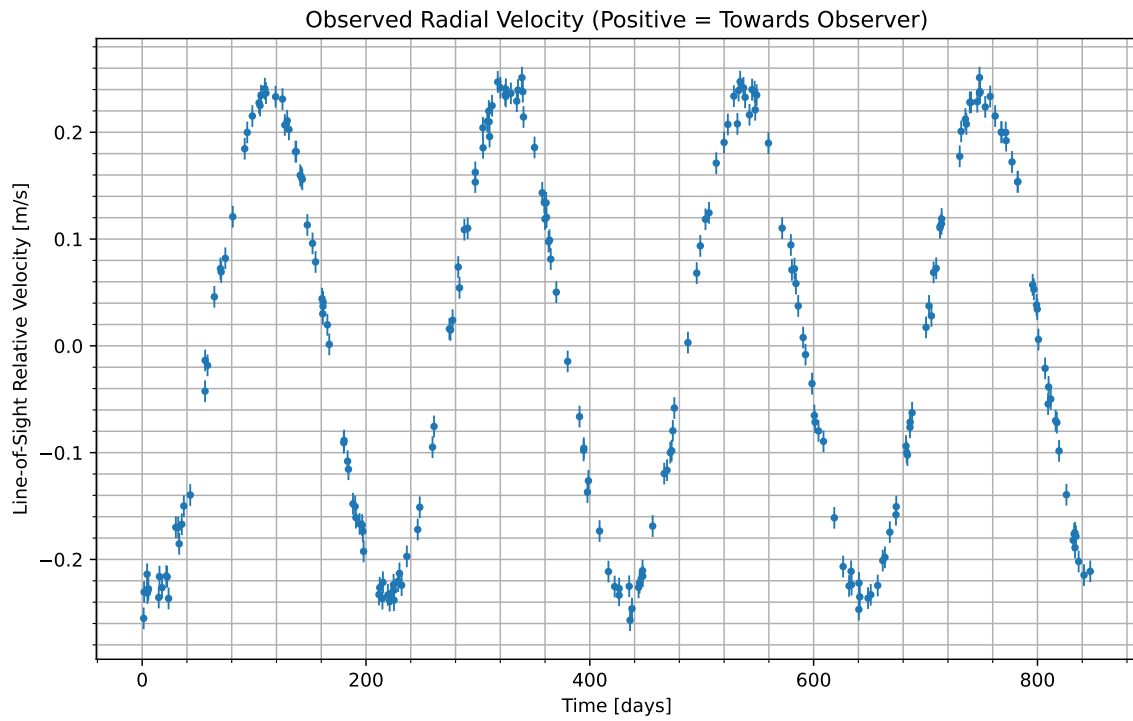
Figure 1: We have isolated the radial velocity of the host star due to the candidate planet. Data begins at UTC 2072-03-06/19:15. Positive values indicate the velocity at which the star is moving towards us; negative indicate the velocity at which it is moving away.
