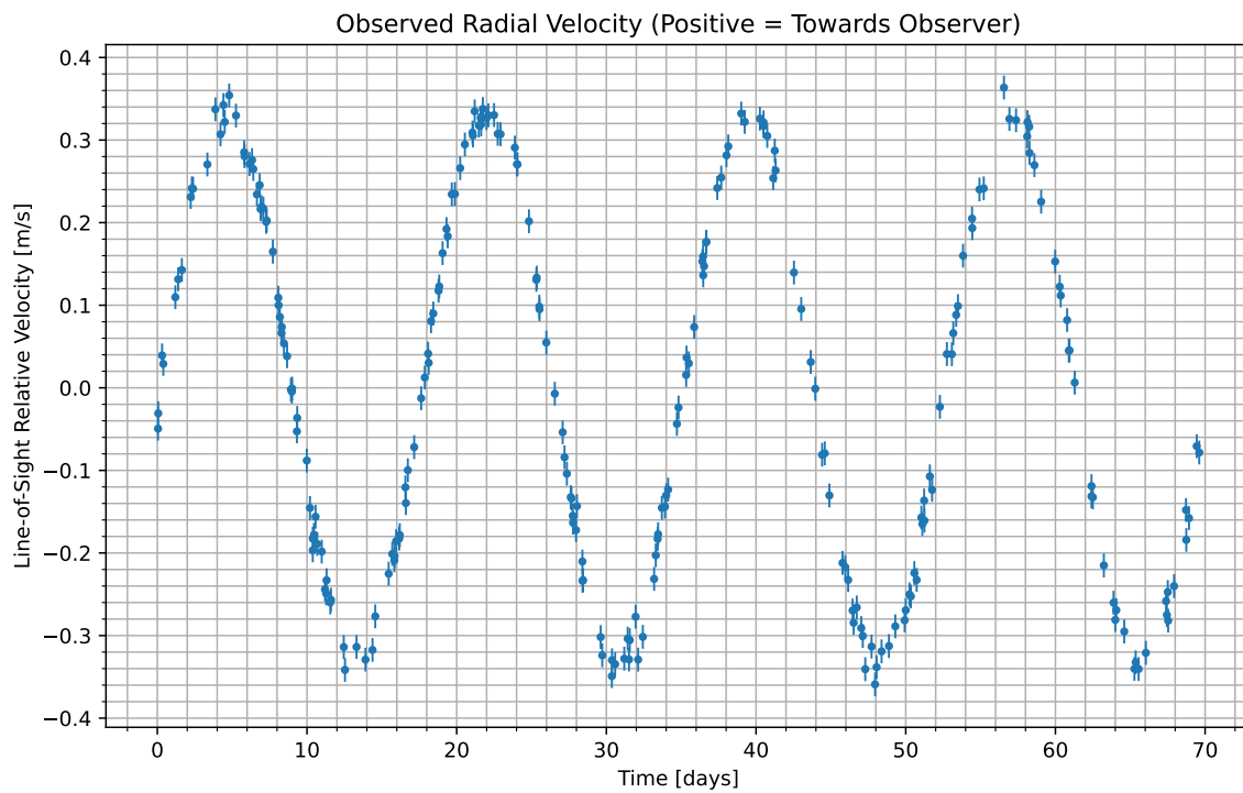
Figure 1: We have isolated the radial velocity of the host star due to the candidate planet. Data begins at UTC 2095-05-15/23:44. Positive values indicate the velocity at which the star is moving towards us; negative indicate the velocity at which it is moving away.
