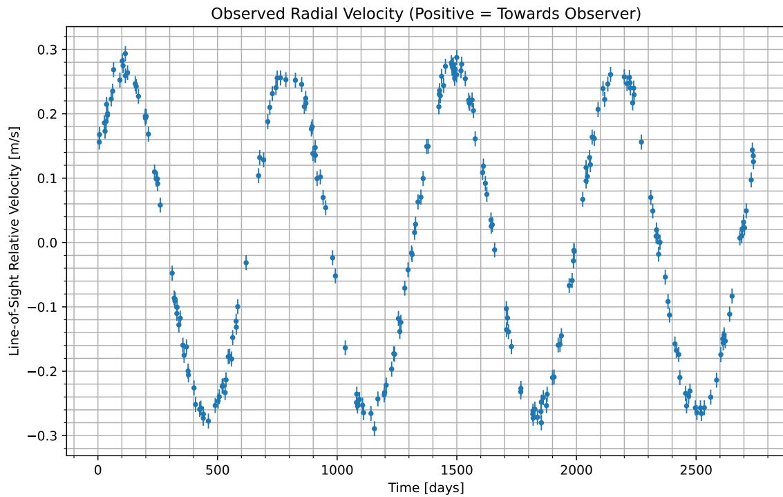
Figure 1: We have isolated the radial velocity of the host star due to the candidate planet. Data begins at UTC 2091-10-18/23:29. Positive values indicate the velocity at which the star is moving towards us; negative indicate the velocity at which it is moving away.
