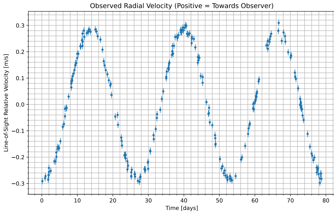
Figure 1: We have isolated the radial velocity of the host star due to the candidate planet. Data begins at UTC 2090-05-06/10:09. Positive values indicate the velocity at which the star is moving towards us; negative indicate the velocity at which it is moving away.
