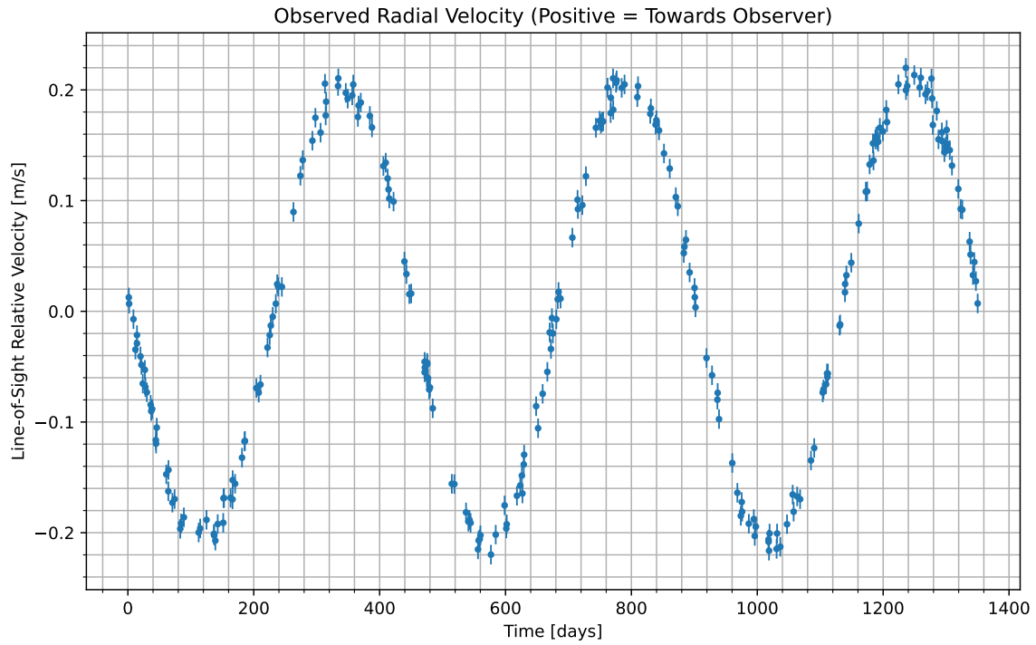
Figure 1: We have isolated the radial velocity of the host star due to the candidate planet. Data begins at UTC 2077-02-06/23:27. Positive values indicate the velocity at which the star is moving towards us; negative indicate the velocity at which it is moving away.
