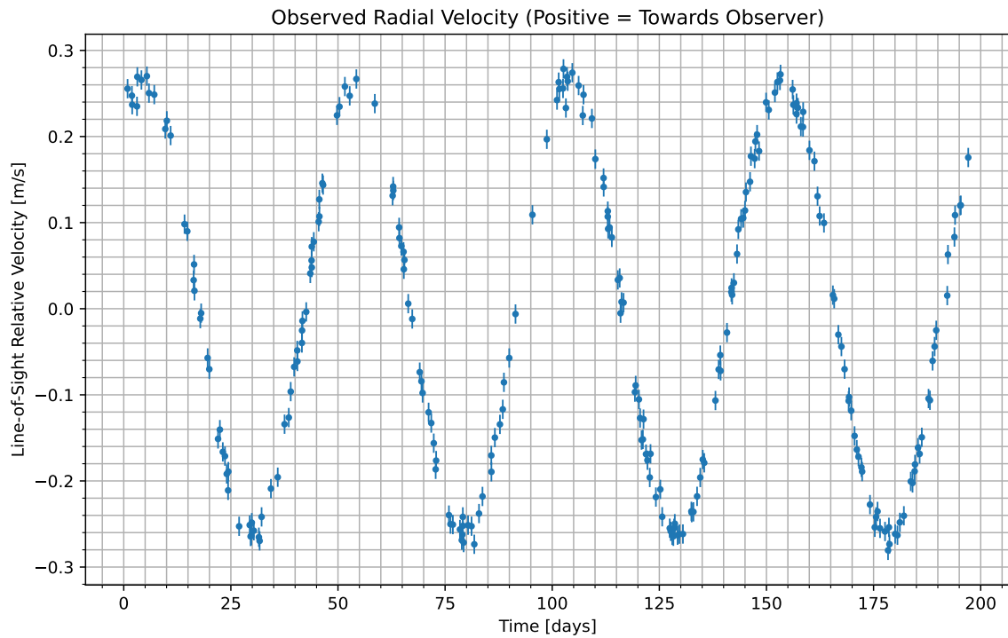
Figure 1: We have isolated the radial velocity of the host star due to the candidate planet. Data begins at UTC 2070-07-30/04:03. Positive values indicate the velocity at which the star is moving towards us; negative indicate the velocity at which it is moving away.
