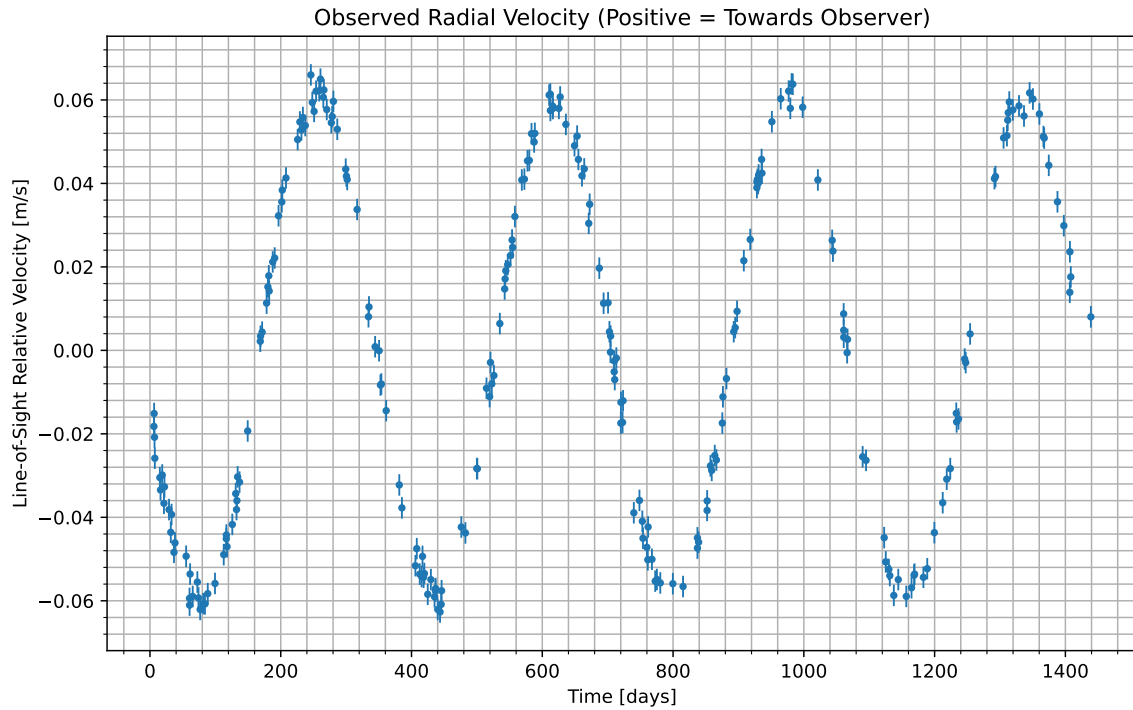
Figure 1: We have isolated the radial velocity of the host star due to the candidate planet. Data begins at UTC 2072-11-14/05:25. Positive values indicate the velocity at which the star is moving towards us; negative indicate the velocity at which it is moving away.
