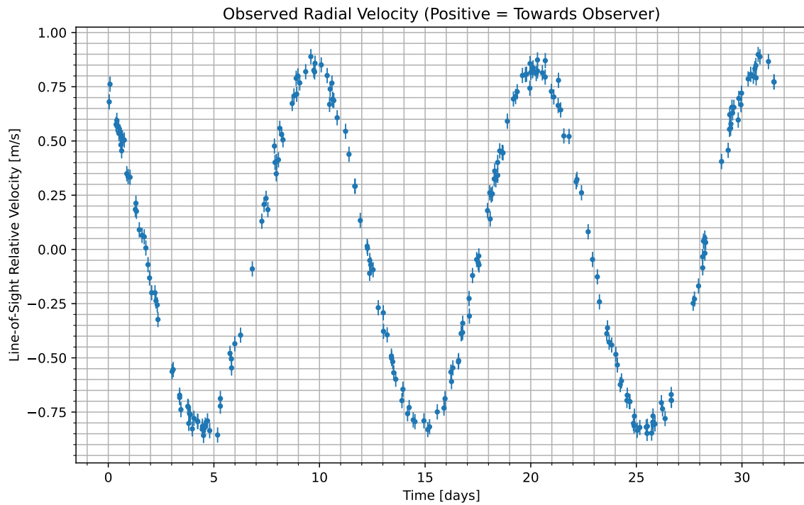
Figure 1: We have isolated the radial velocity of the host star due to the candidate planet. Data begins at UTC 2071-09-19/19:09. Positive values indicate the velocity at which the star is moving towards us; negative indicate the velocity at which it is moving away.
