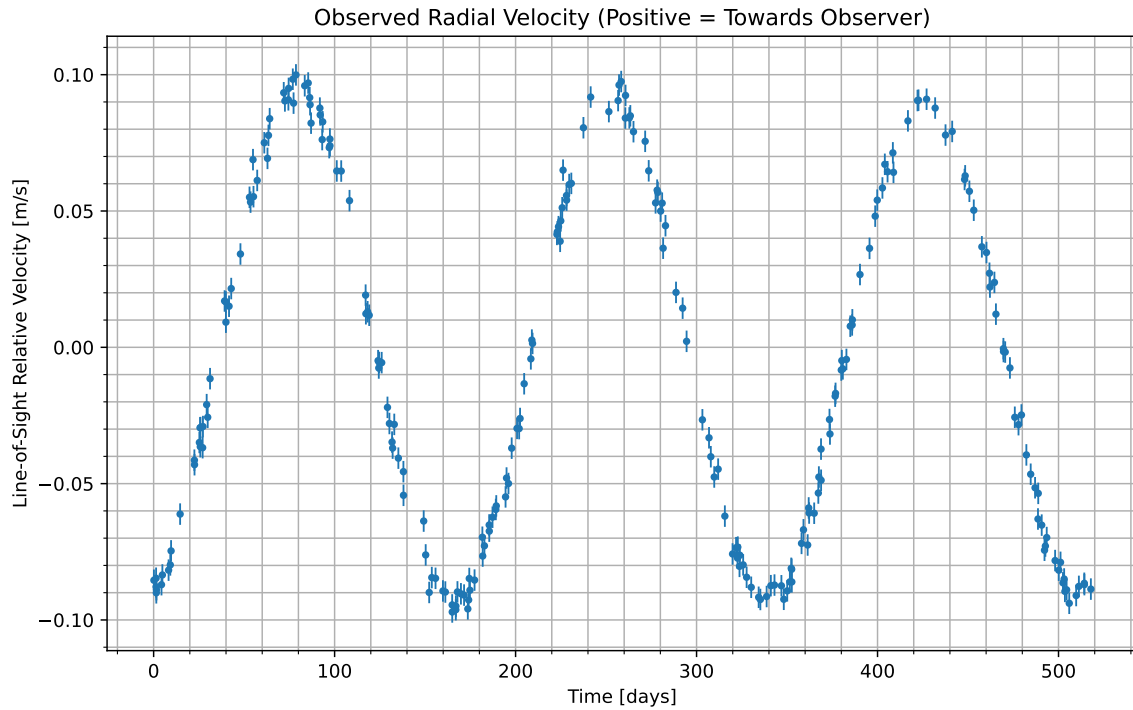
Figure 1: We have isolated the radial velocity of the host star due to the candidate planet. Data begins at UTC 2082-12-07/17:31. Positive values indicate the velocity at which the star is moving towards us; negative indicate the velocity at which it is moving away.
