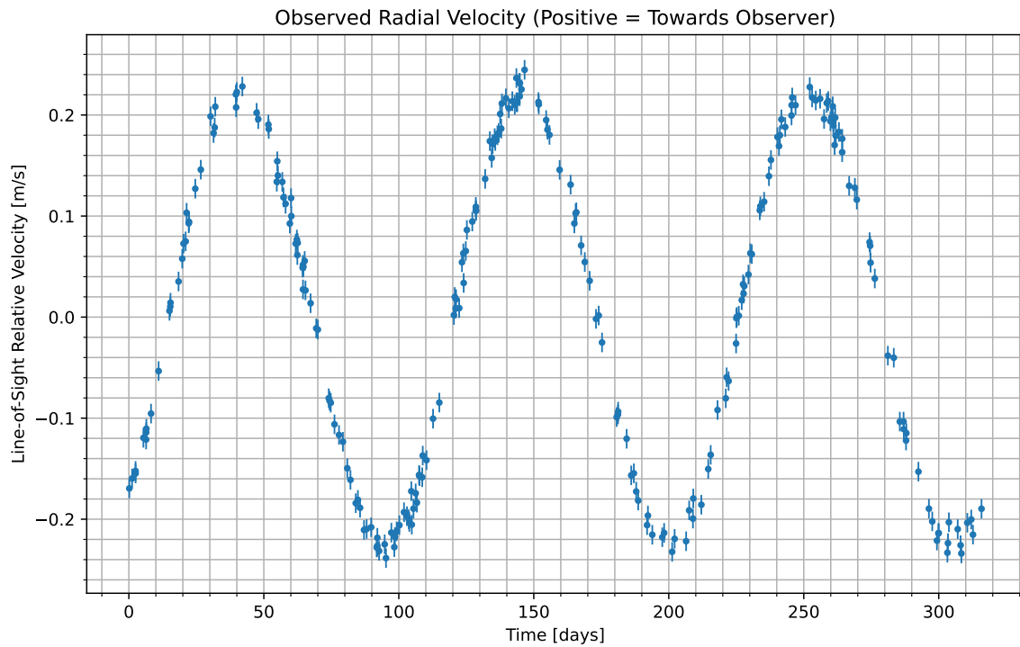
Figure 1: We have isolated the radial velocity of the host star due to the candidate planet. Data begins at UTC 2070-11-19/05:44. Positive values indicate the velocity at which the star is moving towards us; negative indicate the velocity at which it is moving away.
