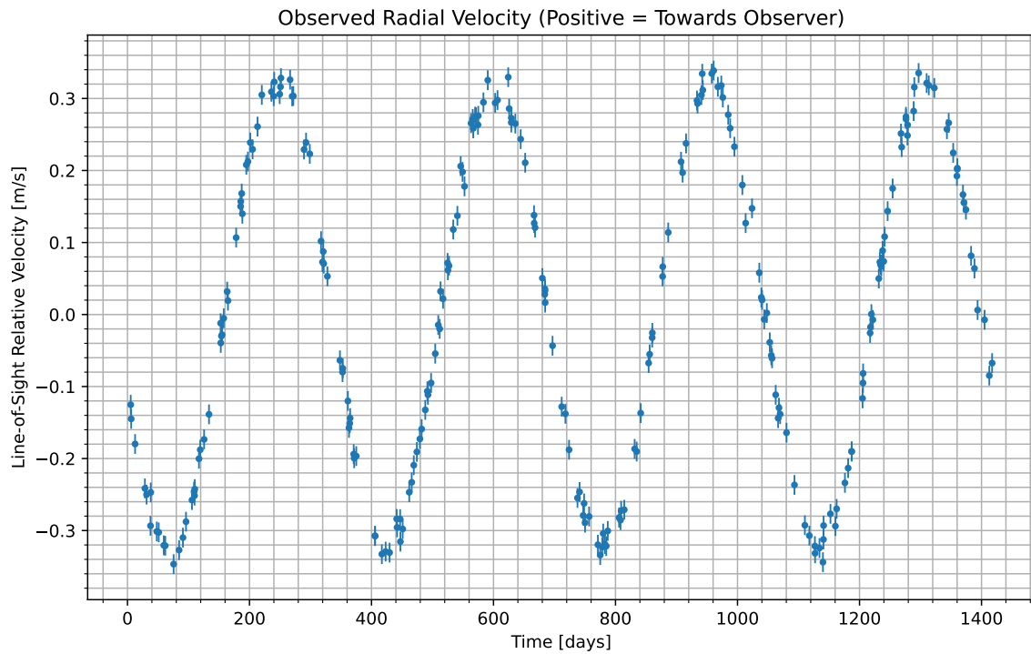
Figure 1: We have isolated the radial velocity of the host star due to the candidate planet. Data begins at UTC 2083-10-03/07:59. Positive values indicate the velocity at which the star is moving towards us; negative indicate the velocity at which it is moving away.
