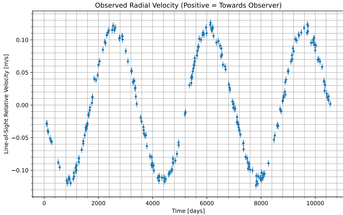
Figure 1: We have isolated the radial velocity of the host star due to the candidate planet. Data begins at UTC 2066-06-13/12:34. Positive values indicate the velocity at which the star is moving towards us; negative indicate the velocity at which it is moving away.
