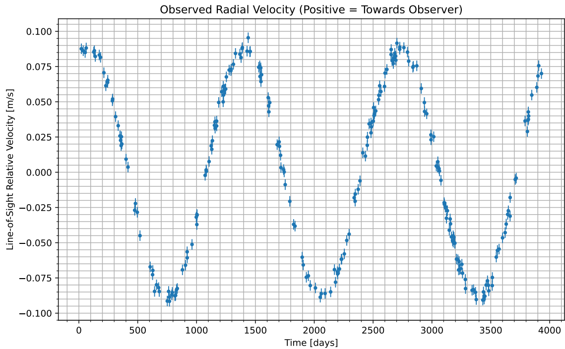
Figure 1: We have isolated the radial velocity of the host star due to the candidate planet. Data begins at UTC 2079-01-13/19:42. Positive values indicate the velocity at which the star is moving towards us; negative indicate the velocity at which it is moving away.
