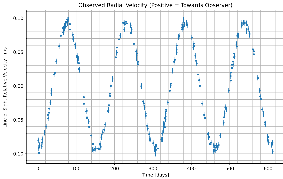
Figure 1: We have isolated the radial velocity of the host star due to the candidate planet. Data begins at UTC 2073-02-11/19:39. Positive values indicate the velocity at which the star is moving towards us; negative indicate the velocity at which it is moving away.
