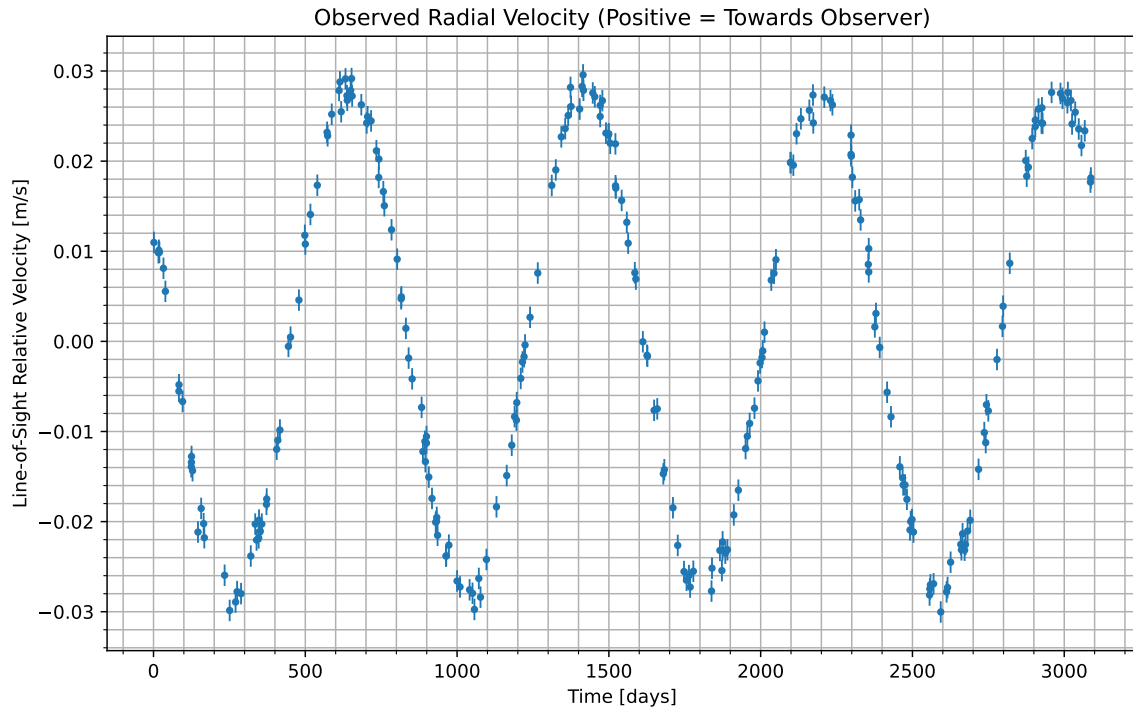
Figure 1: We have isolated the radial velocity of the host star due to the candidate planet. Data begins at UTC 2081-04-25/00:38. Positive values indicate the velocity at which the star is moving towards us; negative indicate the velocity at which it is moving away.
