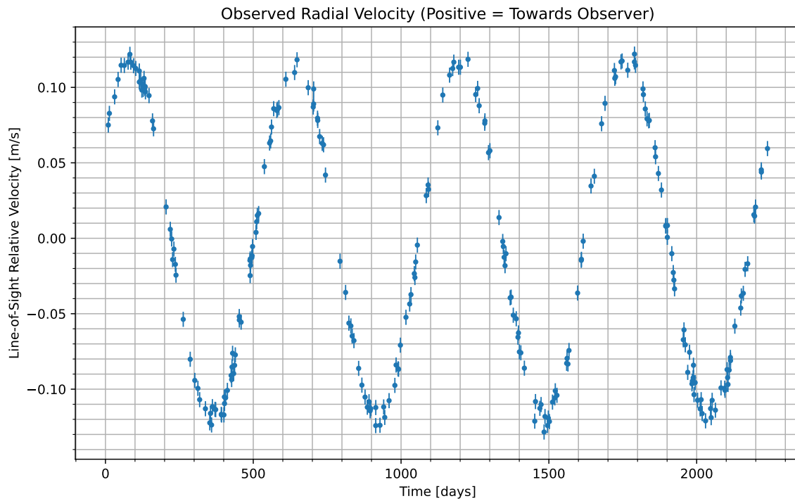
Figure 1: We have isolated the radial velocity of the host star due to the candidate planet. Data begins at UTC 2087-11-18/08:27. Positive values indicate the velocity at which the star is moving towards us; negative indicate the velocity at which it is moving away.
