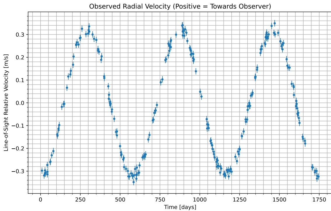
Figure 1: We have isolated the radial velocity of the host star due to the candidate planet. Data begins at UTC 2096-01-07/22:17. Positive values indicate the velocity at which the star is moving towards us; negative indicate the velocity at which it is moving away.
