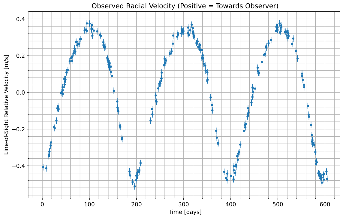
Figure 1: We have isolated the radial velocity of the host star due to the candidate planet. Data begins at UTC 2082-07-29/10:46. Positive values indicate the velocity at which the star is moving towards us; negative indicate the velocity at which it is moving away.
