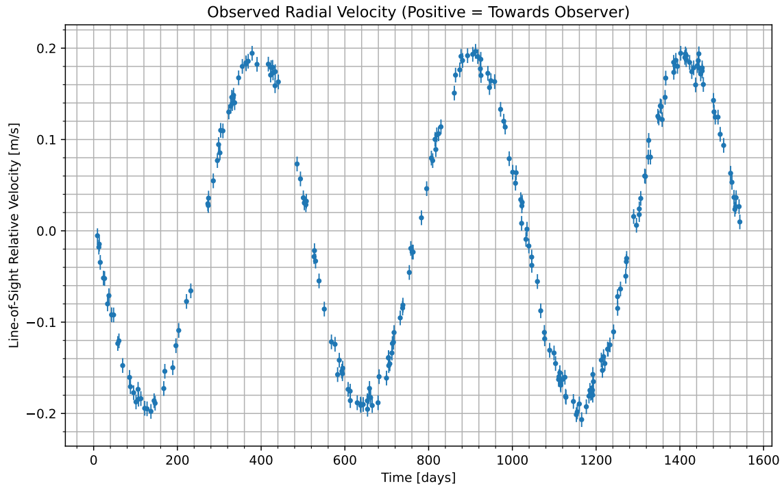
Figure 1: We have isolated the radial velocity of the host star due to the candidate planet. Data begins at UTC 2094-03-20/07:48. Positive values indicate the velocity at which the star is moving towards us; negative indicate the velocity at which it is moving away.
