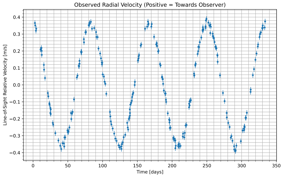
Figure 1: We have isolated the radial velocity of the host star due to the candidate planet. Data begins at UTC 2088-02-14/21:04. Positive values indicate the velocity at which the star is moving towards us; negative indicate the velocity at which it is moving away.
