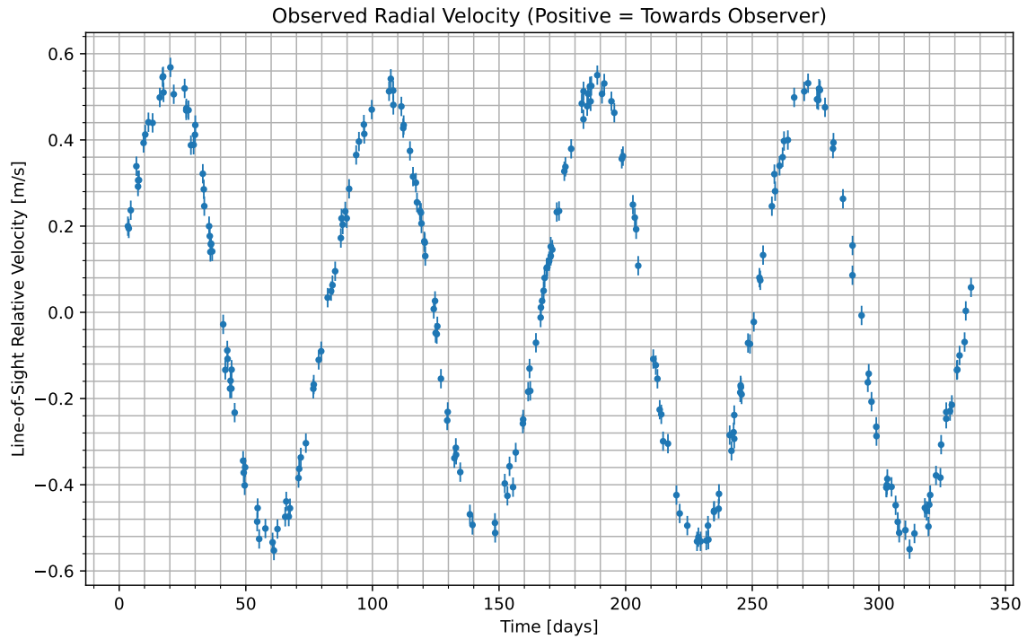
Figure 1: We have isolated the radial velocity of the host star due to the candidate planet. Data begins at UTC 2077-04-22/06:22. Positive values indicate the velocity at which the star is moving towards us; negative indicate the velocity at which it is moving away.
