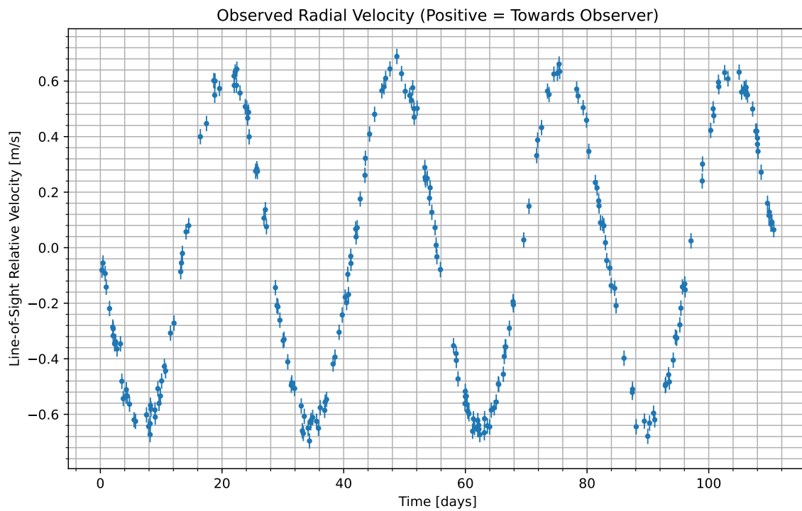
Figure 1: We have isolated the radial velocity of the host star due to the candidate planet. Data begins at UTC 2071-04-12/21:02. Positive values indicate the velocity at which the star is moving towards us; negative indicate the velocity at which it is moving away.
