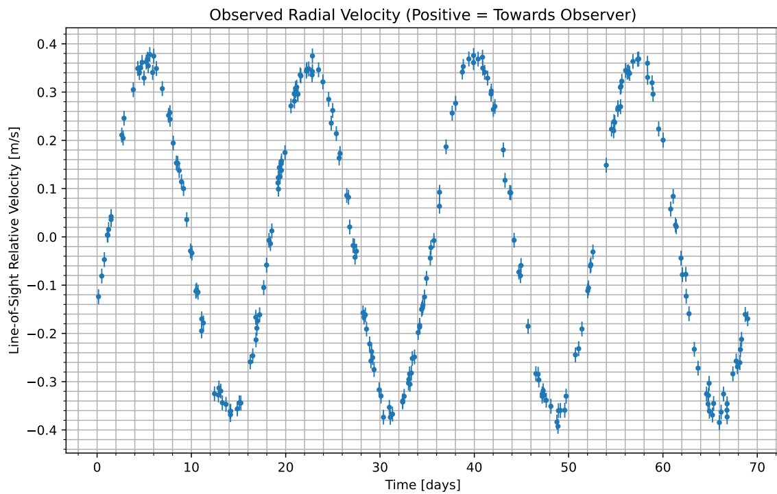
Figure 1: We have isolated the radial velocity of the host star due to the candidate planet. Data begins at UTC 2087-03-05/08:05. Positive values indicate the velocity at which the star is moving towards us; negative indicate the velocity at which it is moving away.
