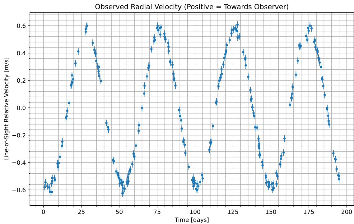
Figure 1: We have isolated the radial velocity of the host star due to the candidate planet. Data begins at UTC 2087-01-25/11:51. Positive values indicate the velocity at which the star is moving towards us; negative indicate the velocity at which it is moving away.
