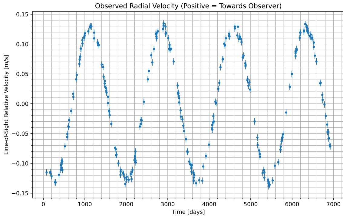
Figure 1: We have isolated the radial velocity of the host star due to the candidate planet. Data begins at UTC 2055-08-03/02:25. Positive values indicate the velocity at which the star is moving towards us; negative indicate the velocity at which it is moving away.
