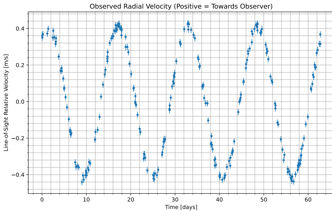
Figure 1: We have isolated the radial velocity of the host star due to the candidate planet. Data begins at UTC 2079-08-19/07:45. Positive values indicate the velocity at which the star is moving towards us; negative indicate the velocity at which it is moving away.
