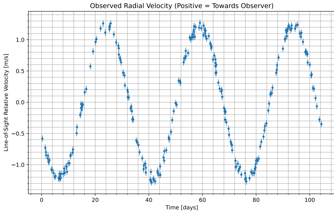
Figure 1: We have isolated the radial velocity of the host star due to the candidate planet. Data begins at UTC 2076-05-25/14:25. Positive values indicate the velocity at which the star is moving towards us; negative indicate the velocity at which it is moving away.
