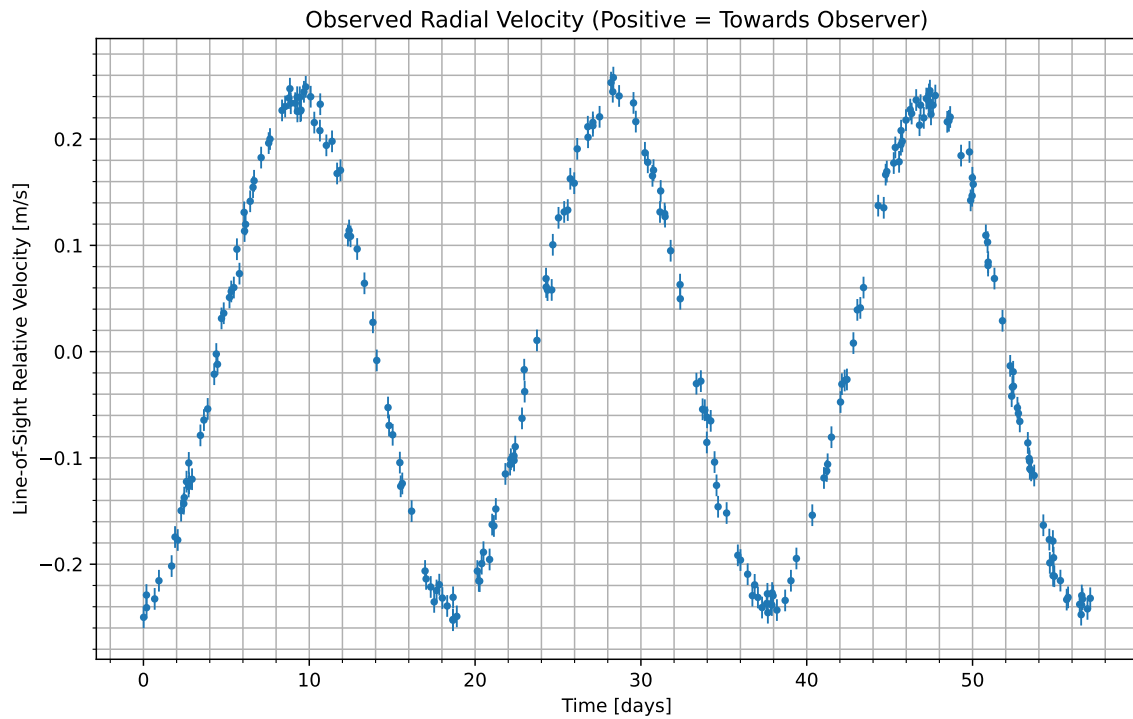
Figure 1: We have isolated the radial velocity of the host star due to the candidate planet. Data begins at UTC 2088-12-22/17:02. Positive values indicate the velocity at which the star is moving towards us; negative indicate the velocity at which it is moving away.
