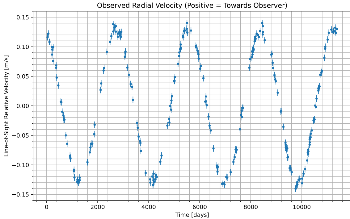
Figure 1: We have isolated the radial velocity of the host star due to the candidate planet. Data begins at UTC 2042-07-27/19:27. Positive values indicate the velocity at which the star is moving towards us; negative indicate the velocity at which it is moving away.
