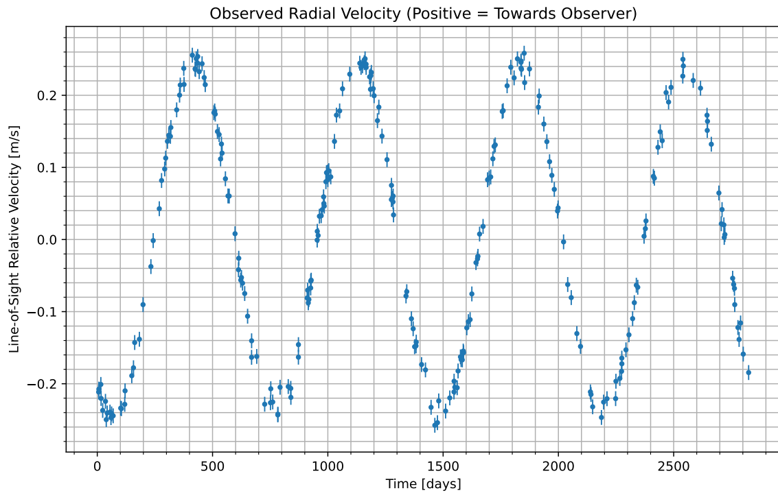
Figure 1: We have isolated the radial velocity of the host star due to the candidate planet. Data begins at UTC 2082-11-19/16:27. Positive values indicate the velocity at which the star is moving towards us; negative indicate the velocity at which it is moving away.
