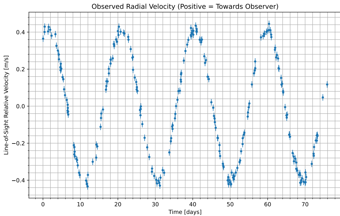
Figure 1: We have isolated the radial velocity of the host star due to the candidate planet. Data begins at UTC 2084-04-07/21:07. Positive values indicate the velocity at which the star is moving towards us; negative indicate the velocity at which it is moving away.
