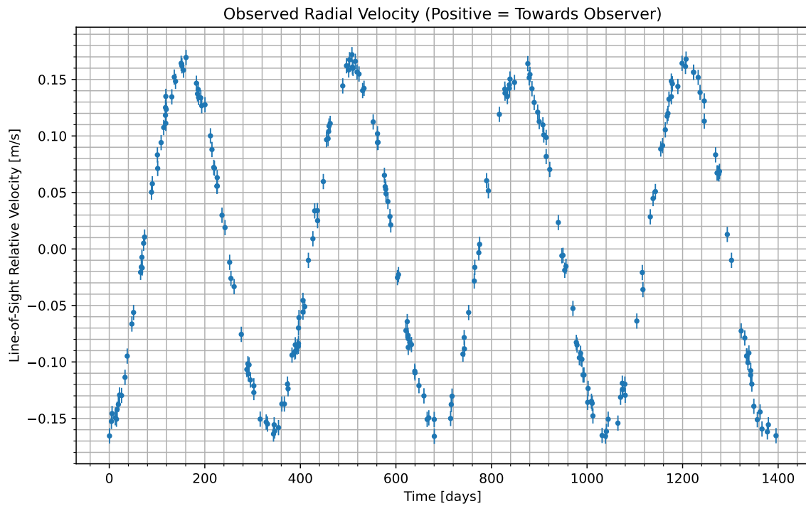
Figure 1: We have isolated the radial velocity of the host star due to the candidate planet. Data begins at UTC 2085-09-25/09:34. Positive values indicate the velocity at which the star is moving towards us; negative indicate the velocity at which it is moving away.
