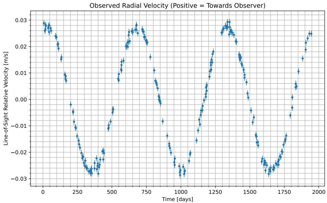
Figure 1: We have isolated the radial velocity of the host star due to the candidate planet. Data begins at UTC 2086-07-30/19:18. Positive values indicate the velocity at which the star is moving towards us; negative indicate the velocity at which it is moving away.
