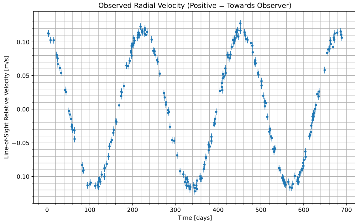
Figure 1: We have isolated the radial velocity of the host star due to the candidate planet. Data begins at UTC 2086-07-26/19:49. Positive values indicate the velocity at which the star is moving towards us; negative indicate the velocity at which it is moving away.
