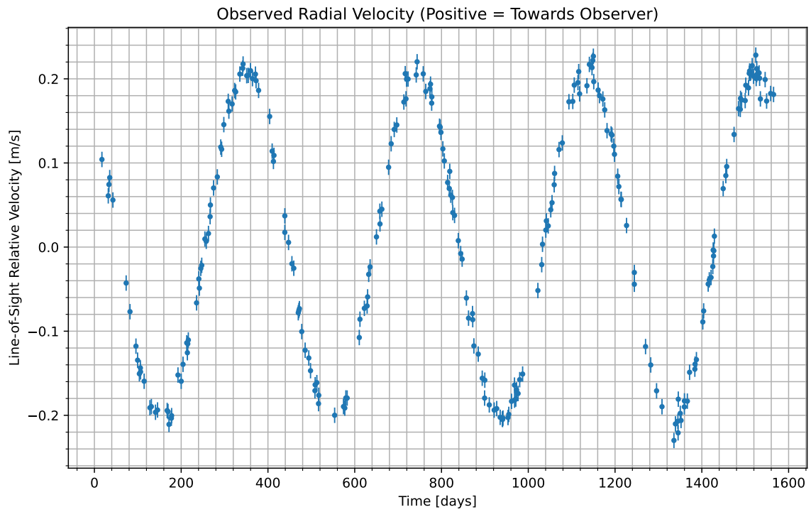
Figure 1: We have isolated the radial velocity of the host star due to the candidate planet. Data begins at UTC 2068-06-13/15:48. Positive values indicate the velocity at which the star is moving towards us; negative indicate the velocity at which it is moving away.
