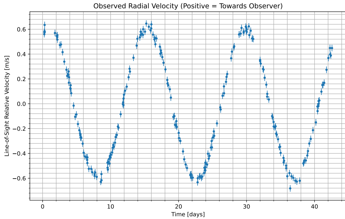
Figure 1: We have isolated the radial velocity of the host star due to the candidate planet. Data begins at UTC 2076-10-09/15:40. Positive values indicate the velocity at which the star is moving towards us; negative indicate the velocity at which it is moving away.
